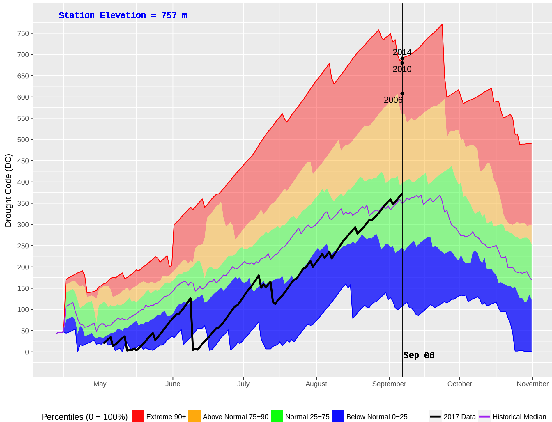
LEMORAY (140) : Historical (1988–2016) and Current (2017) Noon Drought Code (DC)
